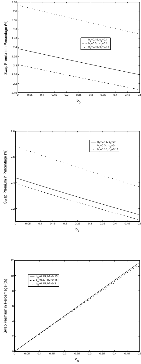
Fig. 1: Swap premium in a two-firm model The protection buyer (firm A) is assumed to be default-free. The swap premium S_2(T) is plotted against various parameters in the contagion risk model, illustrating the impact of the intrinsic and correlated risks of the reference entity and protection seller on the swap premium. The base parameter values are: r = 0.05 , \delta = 0.25 , \Delta T = 0.25 , b_0 = 0.15 , b_2 = 0.15 , c_0 = 0.1 , c_2 = 0.1 , T = 10 .
