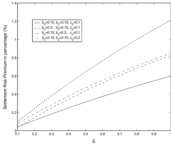
Fig. 2: Change of settlement risk premium on \delta . The base parameter values are: r = 0.05 , \Delta T = 0.25 , b_0 = 0.15 , b_2 = 0.15 , c_0 = 0.1 , c_2 = 0.1 .
