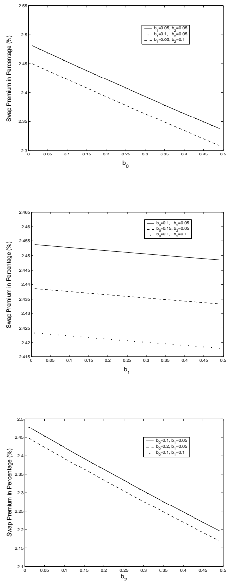
Fig. 4: Impact of risk of default of the protection seller on swap premium. The base parameter values are: r = 0.05 , \delta = 0.25 , \Delta T = 0.25 , T = 10 , a_0 = 0.1 , a_1 = 0.05 , a_2 = 0.05 , b_0 = 0.1 , b_1 = 0.05 , b_2 = 0.05 , c_0 = 0.1 , c_1 = 0.05 , c_2 = 0.05 .
