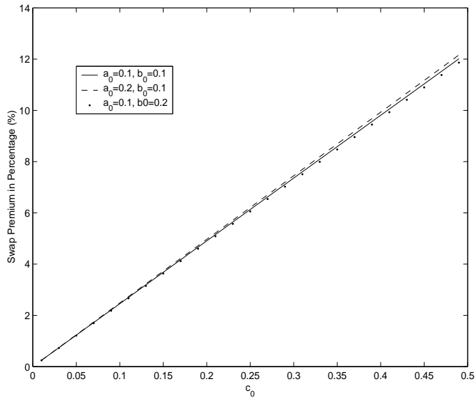
Fig. 3: Impact of risk of default of the protection buyer and the reference entity on swap premium. The base parameter values are: r = 0.05 , \delta = 0.25 , \Delta T = 0.25 , T = 10 , a_0 = 0.1 , a_1 = 0.05 , a_2 = 0.05 , b_0 = 0.1 , b_1 = 0.05 , b_2 = 0.05 , c_0 = 0.1 , c_1 = 0.05 , c_2 = 0.05 .
