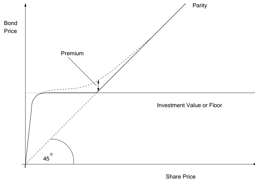
Exhibit 8: Stylized convertible bond price. The thick black line represents the lower bound of the convertible bond price. The lower bound is the parity price for high equity values or the bond floor for lower equity values. The dotted line represents the convertible bond price which trades at a premium to the lower bound in the hybrid region.
