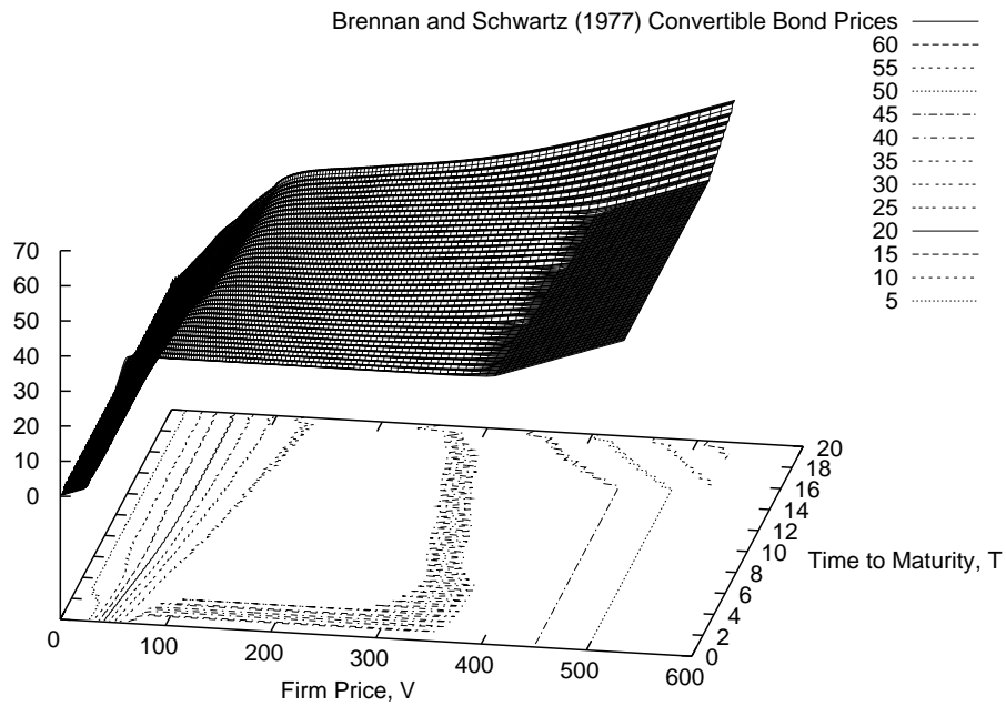
Exhibit 6: Brennan and Schwartz [1977] convertible bond option prices for a contract with par value for the bond of 40, semi-annual coupon of 1.0, quarterly dividend of 1.0, convertible into 10% of the shares outstanding after conversion, firm variance of 0.001 per month, risk free rate of 0.005 per month and with a hard no-call period for the first 5 years followed by a call price of 43 for the next 5 years, 42 for the next five years and 41 for the final 5 years (this example was taken from Brennan and Schwartz [1977]).
