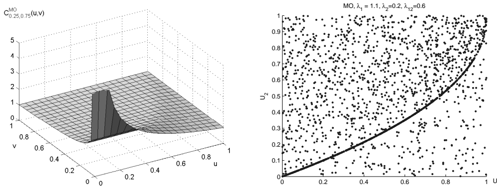
Figure 4: The Marshall-Olkin copula. Left: Continuous part of the density, cut at 5. Right: Simulation of 2000 rvs with a Marshall-Olkin copula. The parameters are \alpha_1 = 0.25 and \alpha_2 = 0.75 or \lambda_1 = 1.1 , \lambda_2 = 0.2 and \lambda_{12} = 0.6 , respectively.
