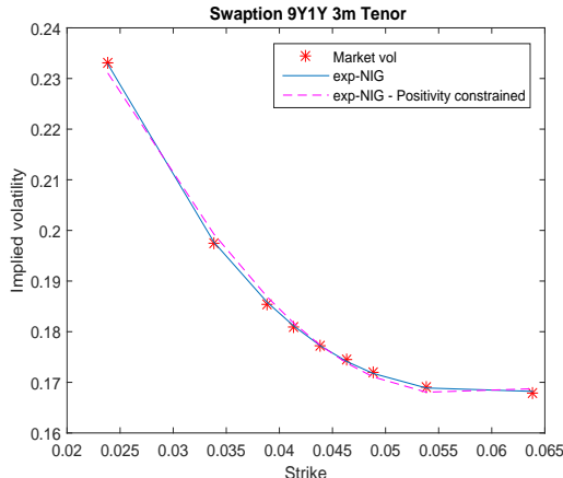
Figure 4: Exponential-NIG calibration
